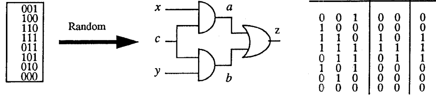
Fig. 6. An example to illustrate the mapping \xi \rightarrow \xi' .
