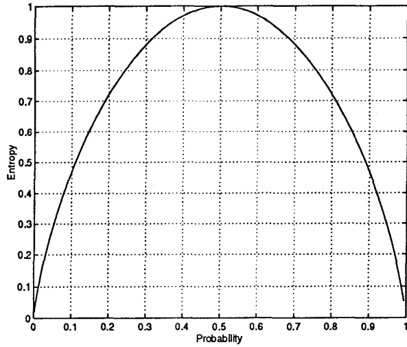
Fig. 2. Entropy H(A_2) versus probability.
